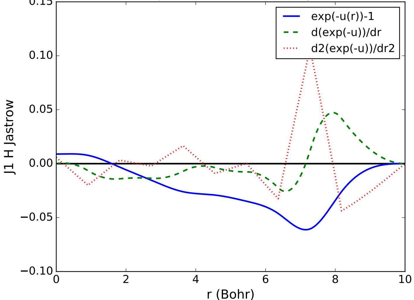
CIPSI-Jastrow/N2H4/N2H4-tr6.wfj.xml
