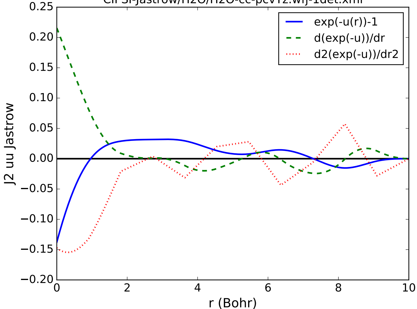
CIPSI-Jastrow/H2O/H2O-cc-pcvTz.wfj-1det.xml
