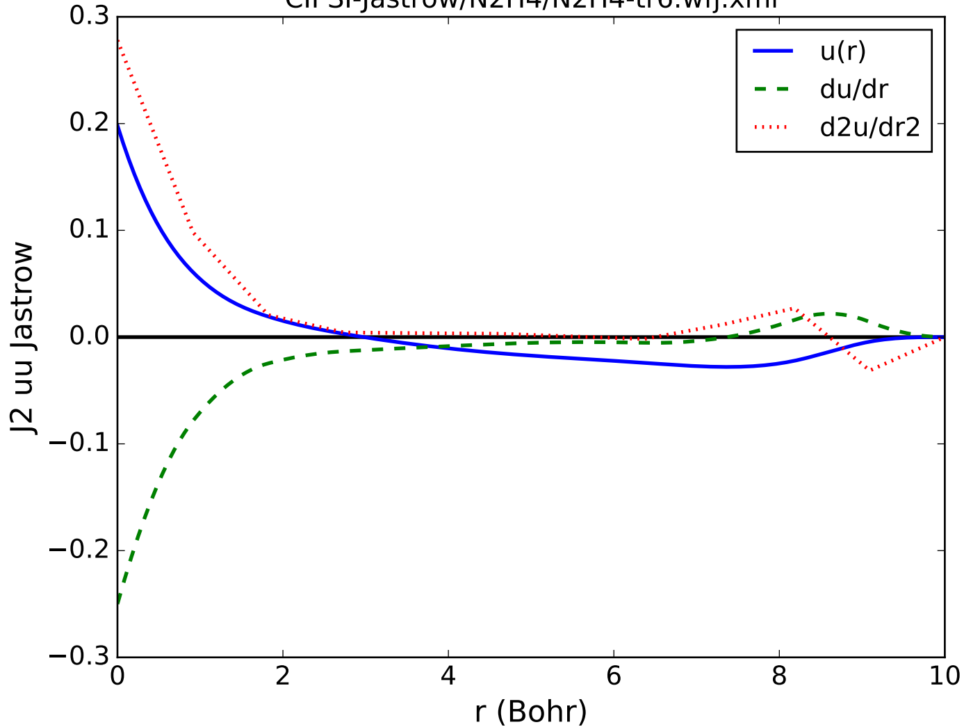
CIPSI-Jastrow/N2H4/N2H4-tr6.wfj.xml
