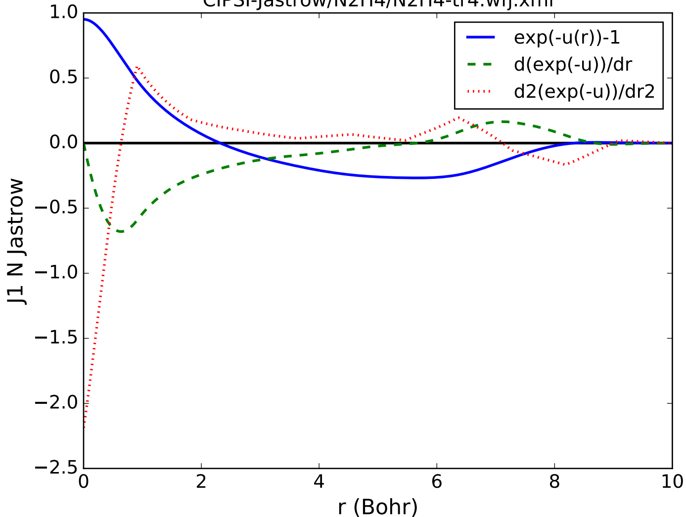
CIPSI-Jastrow/N2H4/N2H4-tr4.wfj.xml
