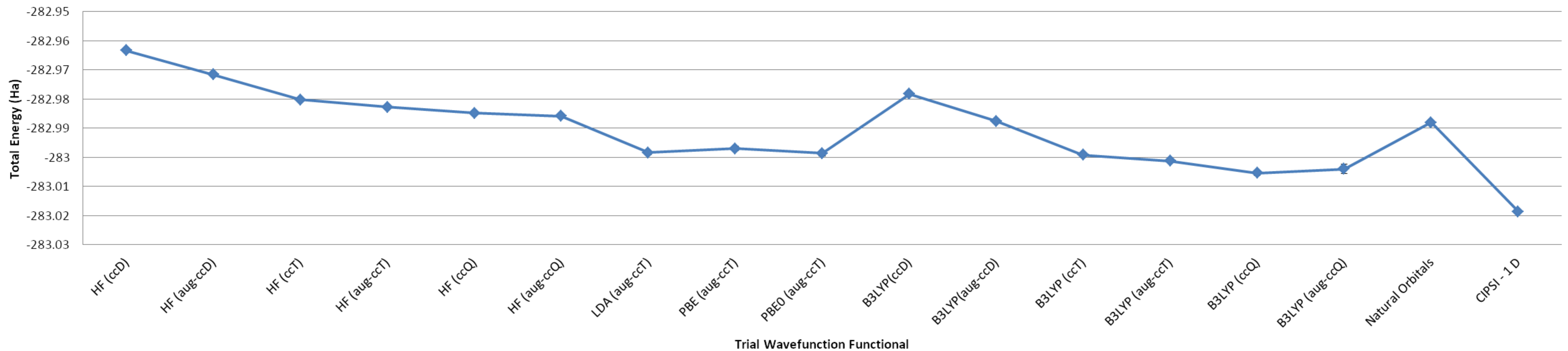
Total energy of Transition as a function of the Trial Wavefunction
