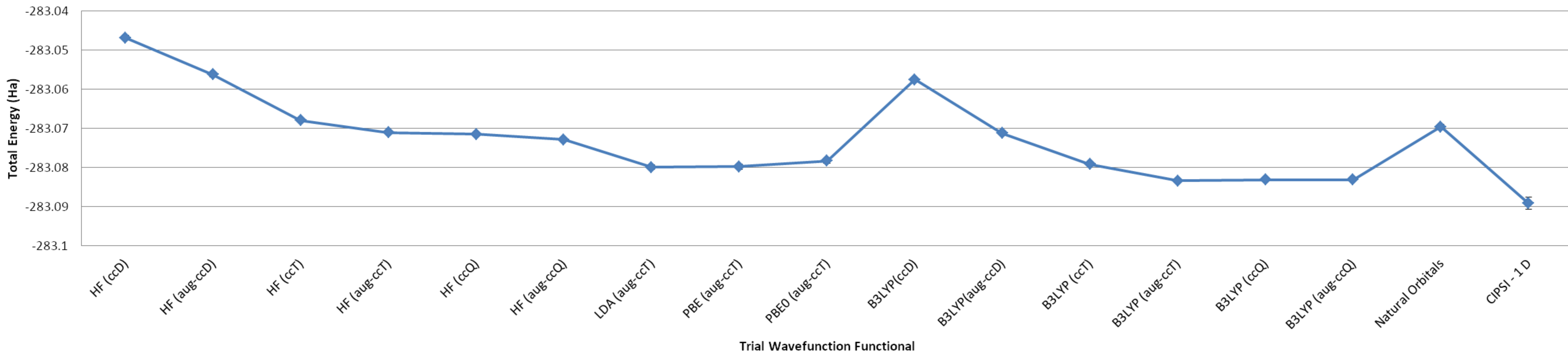
Total energy of Reactants as a function of the Trial Wavefunction
