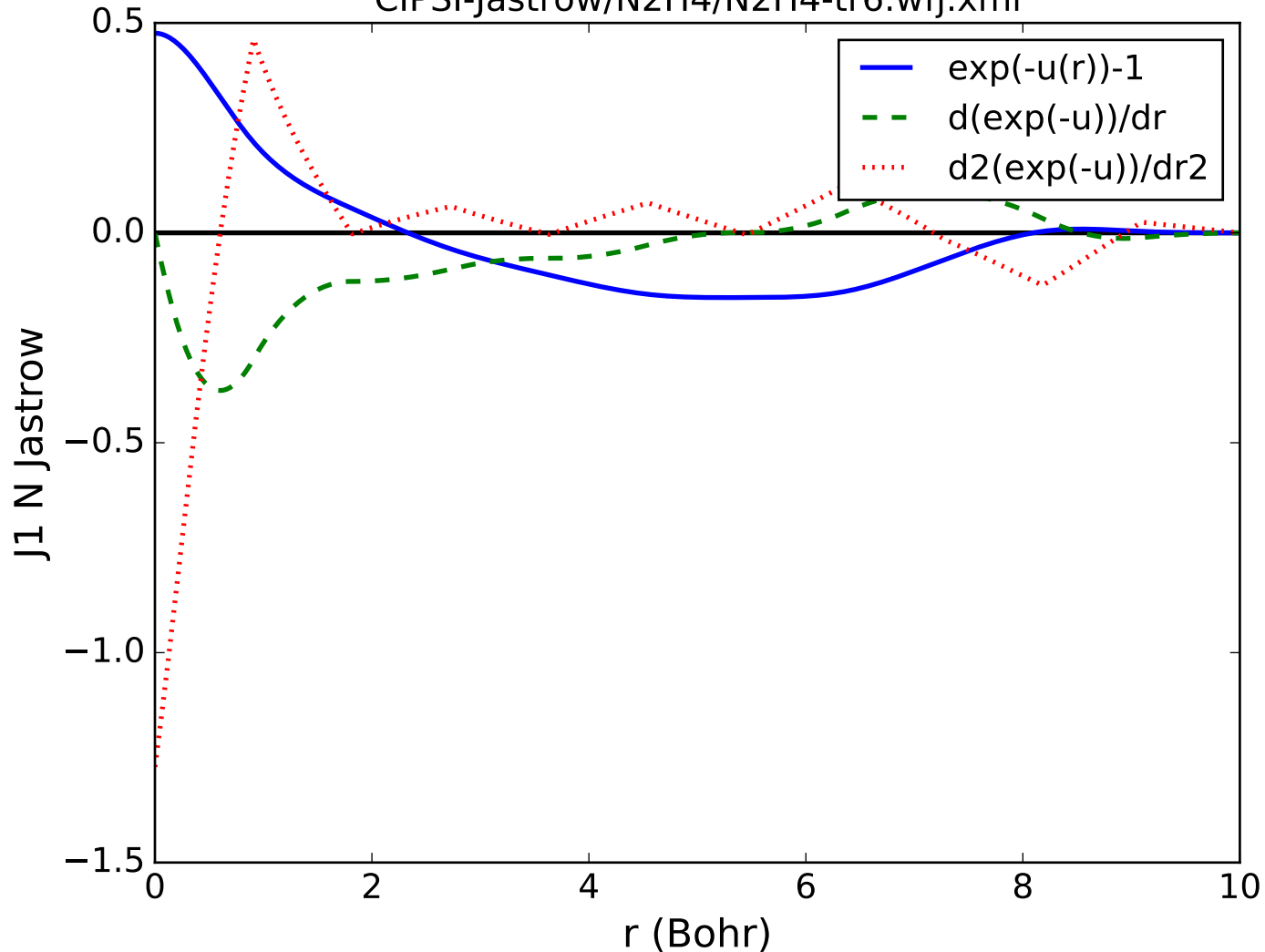
CIPSI-Jastrow/N2H4/N2H4-tr6.wfj.xml
