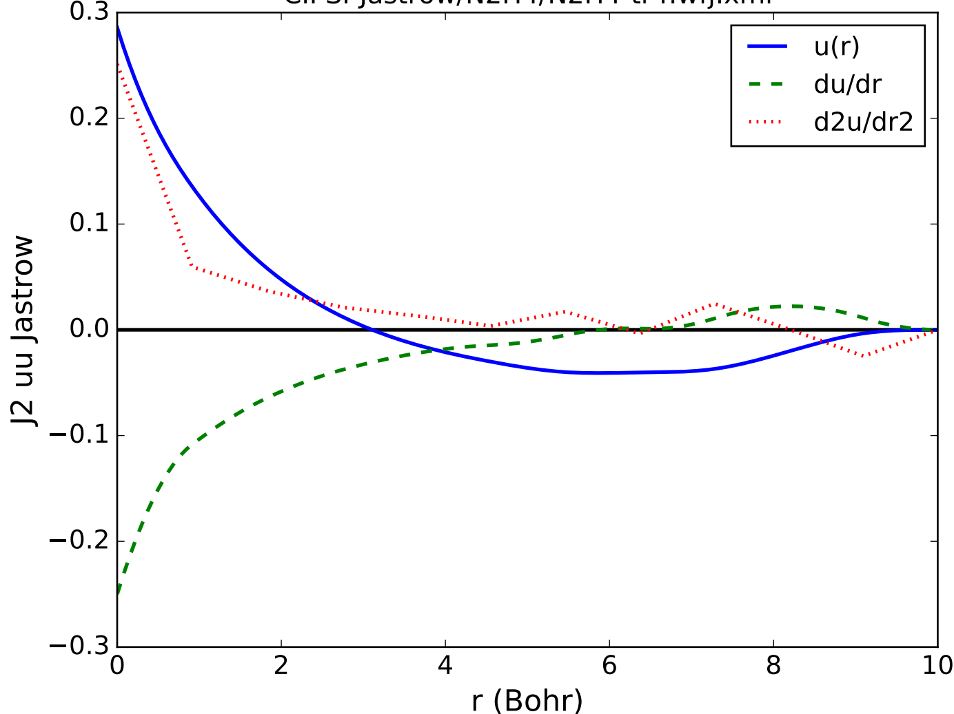
CIPSI-Jastrow/N2H4/N2H4-tr4.wfj.xml
