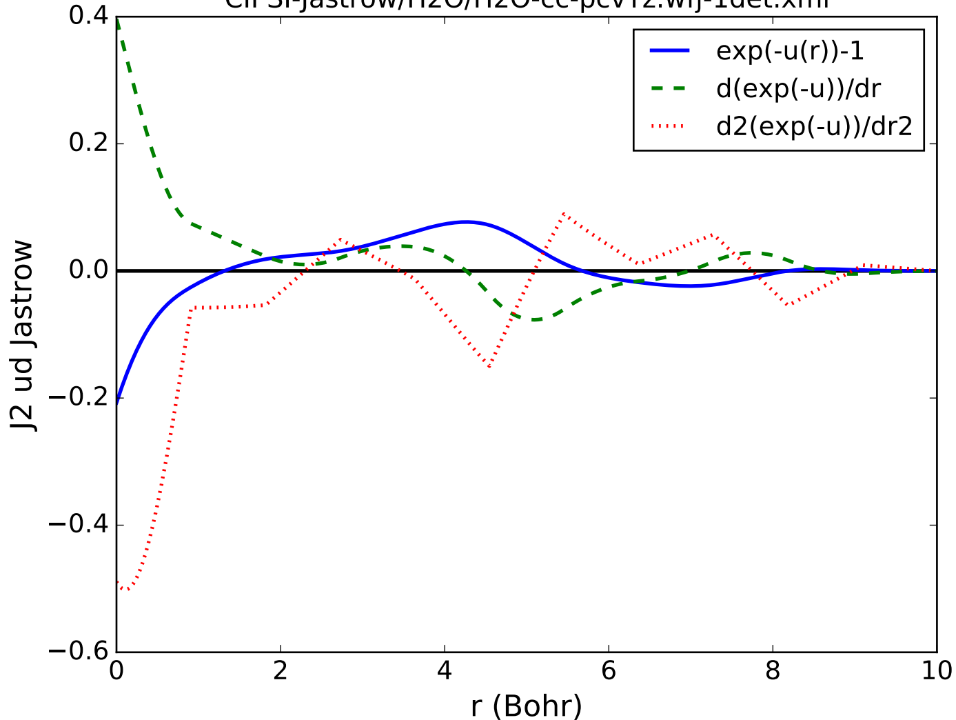
CIPSI-Jastrow/H2O/H2O-cc-pcvTz.wfj-1det.xml
