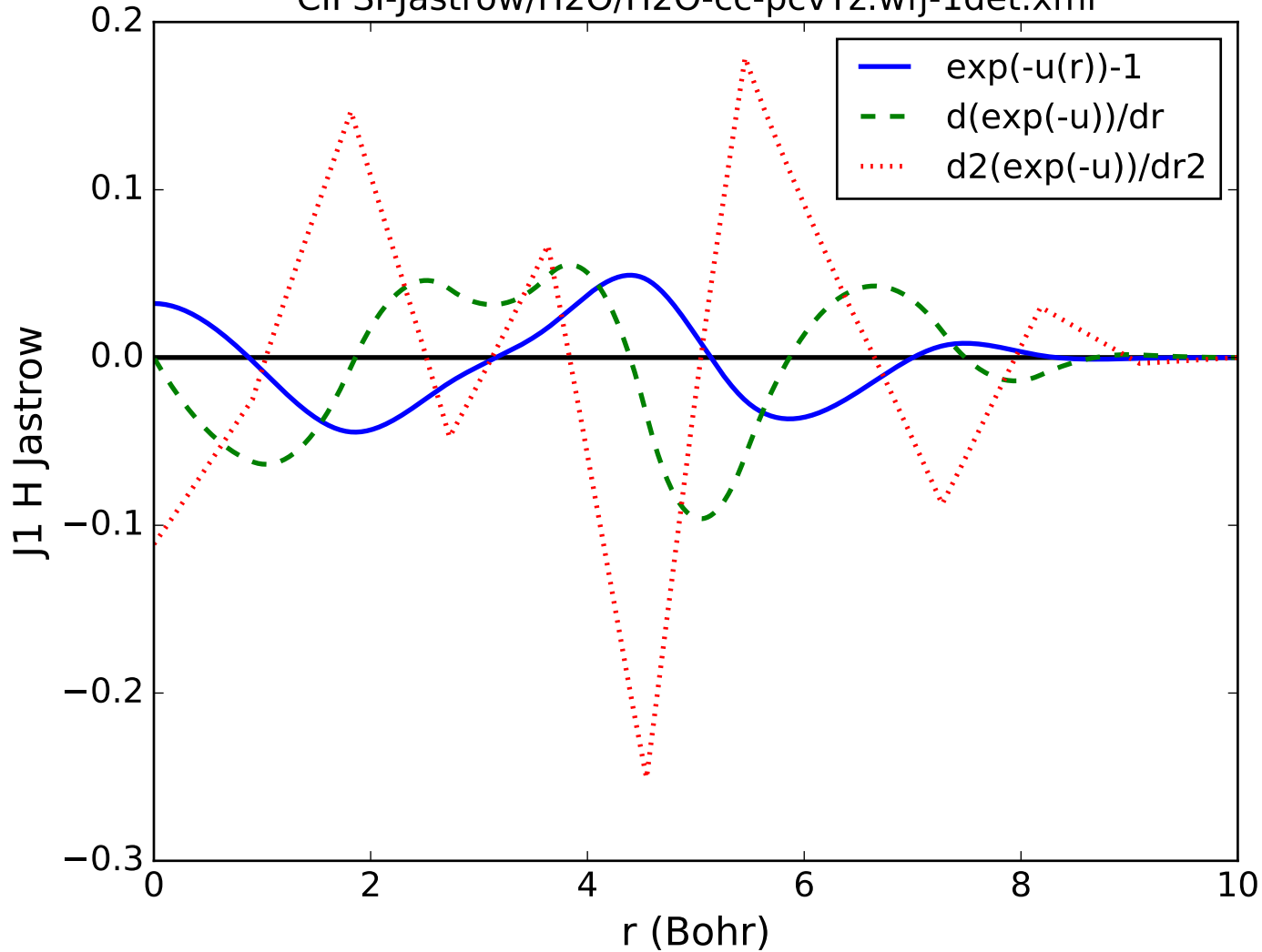
CIPSI-Jastrow/H2O/H2O-cc-pcvTz.wfj-1det.xml
