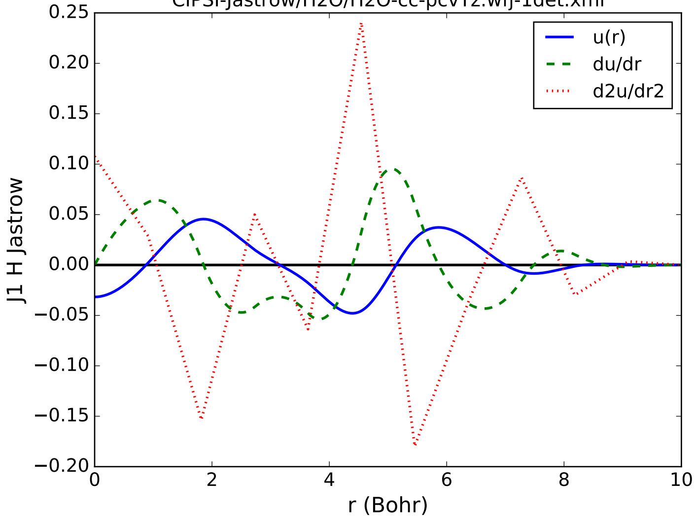
CIPSI-Jastrow/H2O/H2O-cc-pcvTz.wfj-1det.xml
