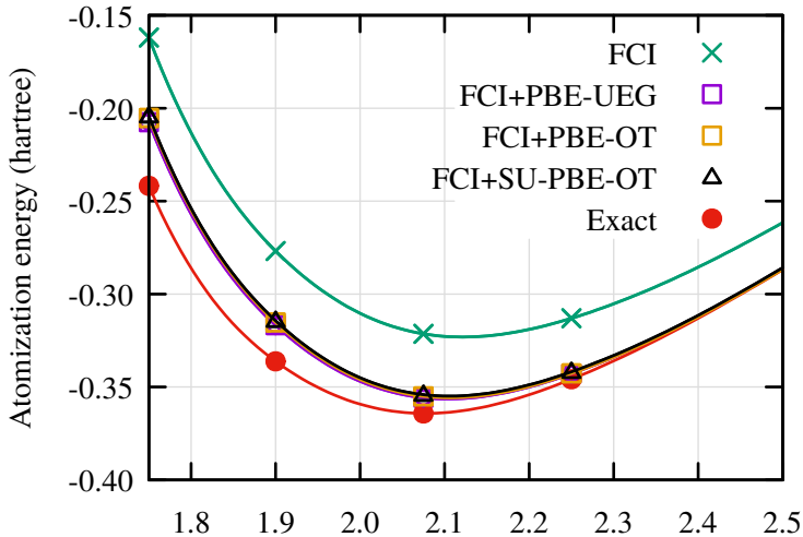
b) N_2 , aug-cc-pVDZ Internuclear distance (bohr)
