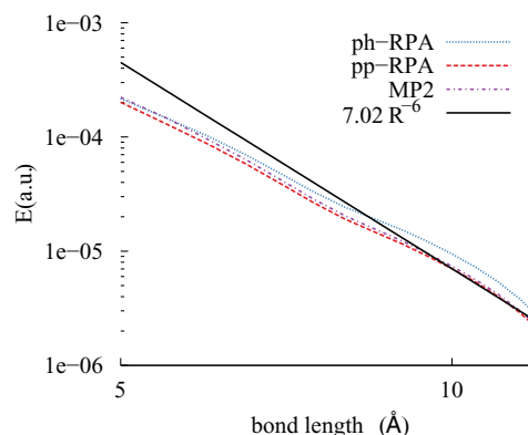
FIG. 6. The pp-RPA interaction energy for the Ar dimer has an R^{-6} decay, very similar to the second order energy in MP2, plotted here on a log-log scale alongside an illustrative R^{-6} function.
