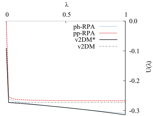
FIG. 3. For two H atoms separated by 10 000 Å the pp-RPA and the ph-RPA correctly reproduce the strong static correlation energy, given by the area under their respective curves. The area under the v2DM* curve shows the exact correlation energy and the v2DM curve shows an approximate constant-density path.
