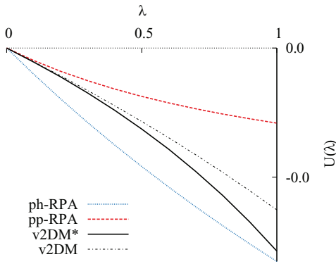
FIG. 1. In H_2 near equilibrium, the pp-RPA slightly underestimates the correlation energy, given by the area under the curve of U(\lambda) along the constant-density path, Eq. (25). The v2DM* curve shows the exact correlation energy, obtained by the adiabatic connection of Eq. (28), while the v2DM curve assumes a constant-density along the path as an approximation, Eq. (27).
