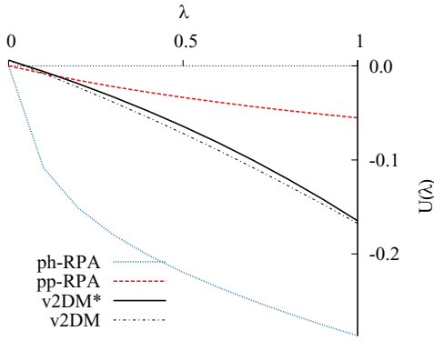
FIG. 5. The pp-RPA correctly produces a small correlation energy for \text{He}_2^+ at 10 Å, given by the area under the curve, while the ph-RPA adds such a large correlation energy to the exact exchange that it fails to bind \text{He}_2^+ . The area under the v2DM* curve shows the exact correlation energy and the v2DM curve shows an approximate constant-density path.
