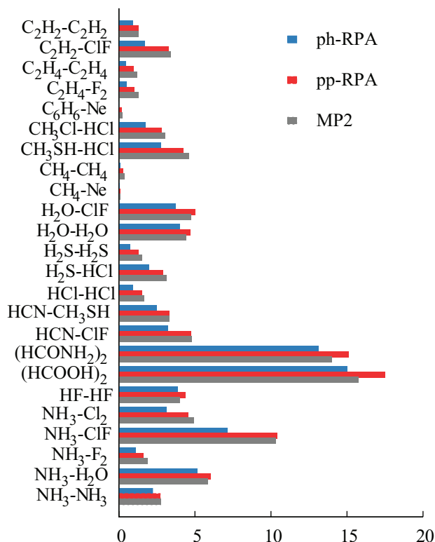
FIG. 8. The (counter-poise corrected) pp-RPA interaction energies (in kcal/mol) are very similar to the MP2 interaction energies for a set of van der Waals bonded molecules.
