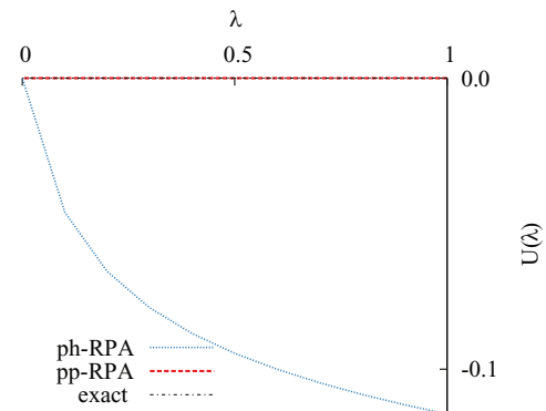
FIG. 4. The pp-RPA correctly adds no correlation energy to the exact exchange in H_2^+ at 10 Å and is thus self-interaction free, while the ph-RPA has a large self-interaction error, given by the area under its curve.
