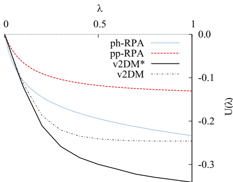
FIG. 2. In H_2 at 10 Å the pp-RPA and the ph-RPA significantly underestimate the correlation energy, given by the area under their respective curves, leading to the unphysical barrier in the dissociation graph for H_2 . The area under the v2DM* curve shows the exact correlation energy and the v2DM curve shows an approximate constant-density path.
