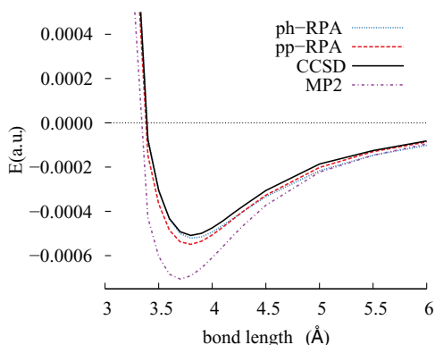
FIG. 7. The pp-RPA and the ph-RPA describe the van der Waals interactions in the Ar dimer well. MP2 binds the dimer more strongly.
