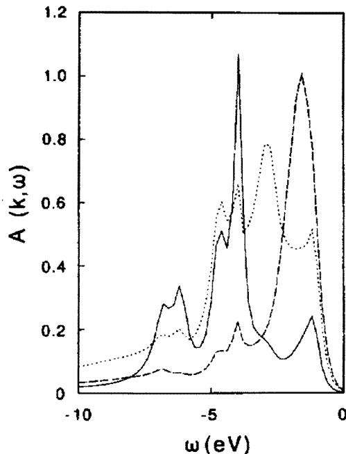
Figure 12. The spectral function of antiferromagnetic NiO at k = \frac{2}{3}(1, 0, 0)2\pi/a within the GWA projected on the O p orbitals (full curve) and the Ni d orbitals (the dotted curve corresponds to the majority spin and the dashed curve the minority spin). After Aryasetiawan and Gunnarsson (1995).
