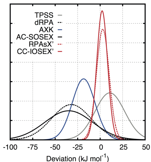
FIG. 1. Normalized Gaussian distributions of deviations from the HEAT benchmark values.
