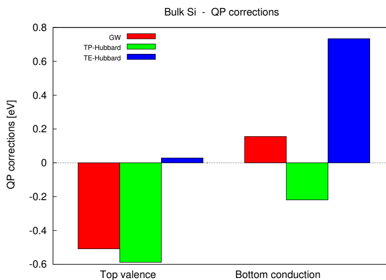
Figure 4.14: Quasiparticle correction at the \Gamma point (0.0;0.0;0.0) in bulk Si for top valence and bottom conduction. GW and Hubbard are compared. The trend of the TE calculation is similar to the TE-ALDA one: the band-gap shift is slightly larger. The TP case is quite different from ALDA and from the large- q HEG kernel, in that both valence and conduction have a negative quasiparticle correction.
