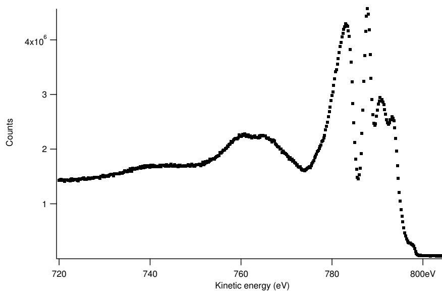
Figure 7.7: Raw XPS spectrum of bulk SiC-4H with single-layer graphene grown on top. The photoelectrons are detected at normal emission and the signal is integrated over an angle of about 6°. The Fermi energy is at 800 eV. With this configuration and at this photon energy, the spectrum is virtually indistinguishable from bulk SiC.
