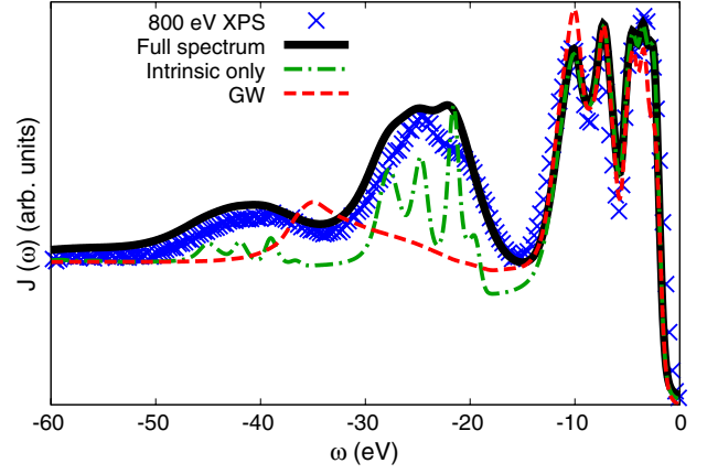
FIG. 1 (color online). Experimental XPS spectrum of Si at 800 eV photon energy (blue crosses), compared to the theoretical intrinsic A(\omega) calculated from G_0 W_0 (red dashed line), and from Eq. (4) (green dot-dashed line). On top of the latter the black solid line also includes extrinsic and interference effects. All spectra contain photoabsorption cross sections, a calculated secondary electron background and 0.4 eV Gaussian broadening to account for finite k -point sampling and experimental resolution. The Fermi energy is set to 0 eV.
