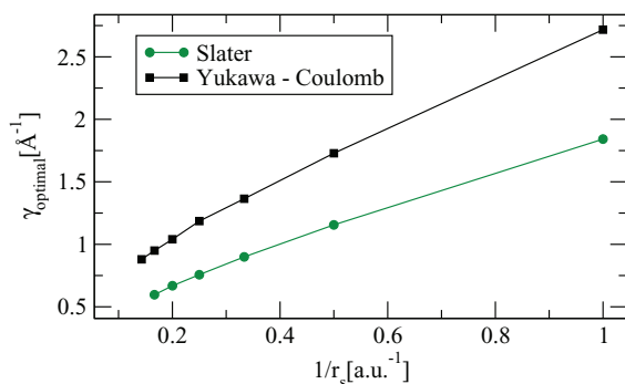
FIG. 7. Change in optimal \gamma parameter for the Slater- and Yukawa-Coulomb correlation factors as the density ( \alpha r_s ) of the electron gas is varied, for the 54 electron simulation cell.
