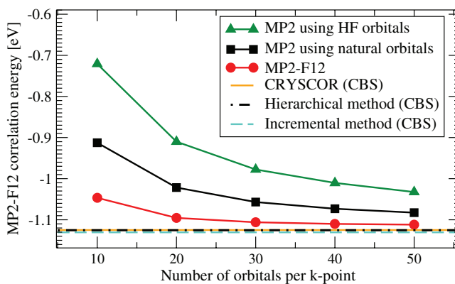
FIG. 13. Basis set convergence of the MP2 valence-only cohesive energy contribution to LiH. Our calculations were done using a 4 \times 4 \times 4 k -mesh and norm-conserving pseudo-potentials in the framework of the PAW method. 76 The LiH unit cell volume was set to 17.03 \text{ \AA}^3 . The MP2 calculations were done using HF and approximate natural orbitals. 12 Our MP2 and MP2-F12 (using a STG) results converge to the same complete basis set limit results obtained using local MP2 (CRYSCOR, from Ref. 13), the hierarchical method (from Ref. 8), and the incremental scheme (from Ref. 14).
