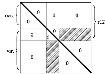
FIG. 1. Scheme of the Fock matrix entering the CC-R12 equations. Note that only the diagonal and the hatched blocks are nonzero.
