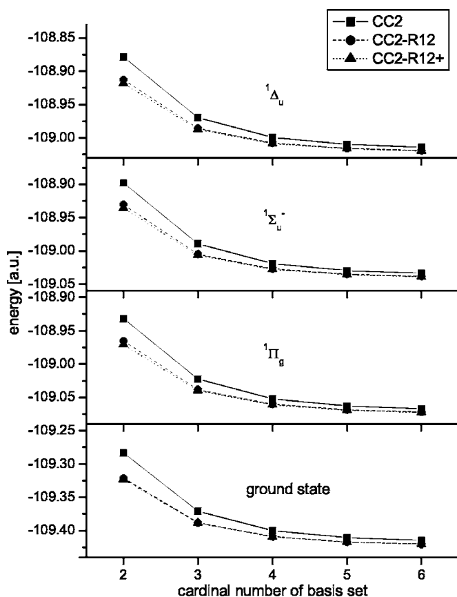
FIG. 5. Basis set dependence of ground and excited states of N_2 (Ansatz 1, approximation B).
