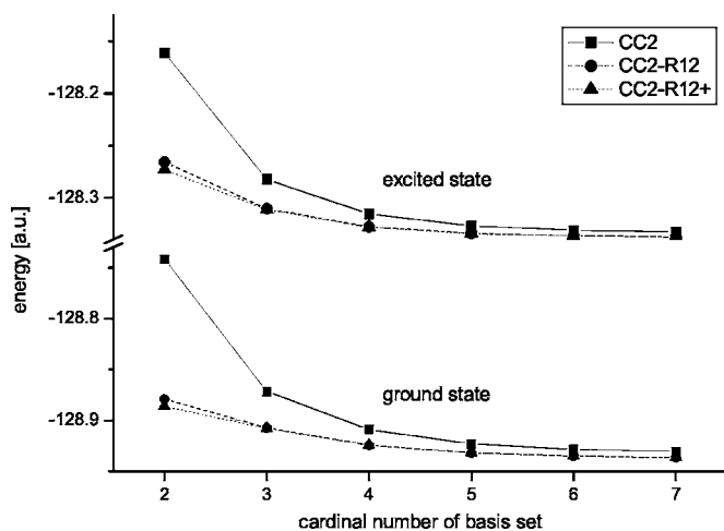
FIG. 3. Basis set dependence of ground and the ^1P ( 3s \leftarrow 2p ) excited state of Ne ( Ansatz 1, approximation B).
