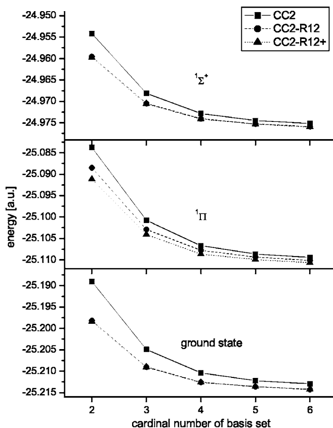
FIG. 4. Basis set dependence of ground and excited states of BH ( Ansatz 1, approximation B).
