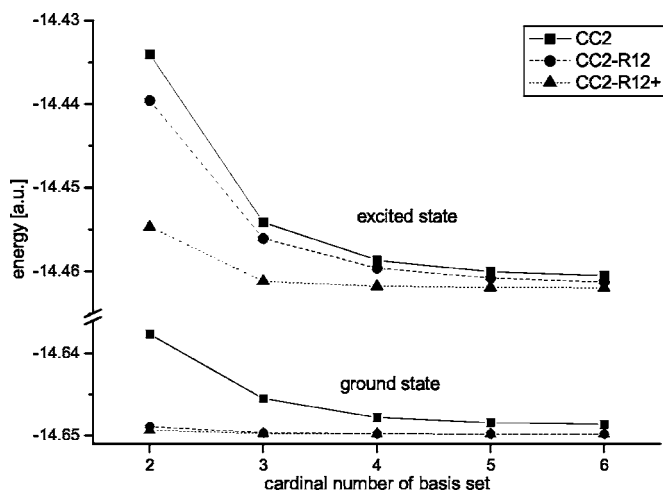
FIG. 2. Basis set dependence of ground and the ^1P ( 2p \leftarrow 2s ) excited state of Be ( Ansatz 1, approximation B).
