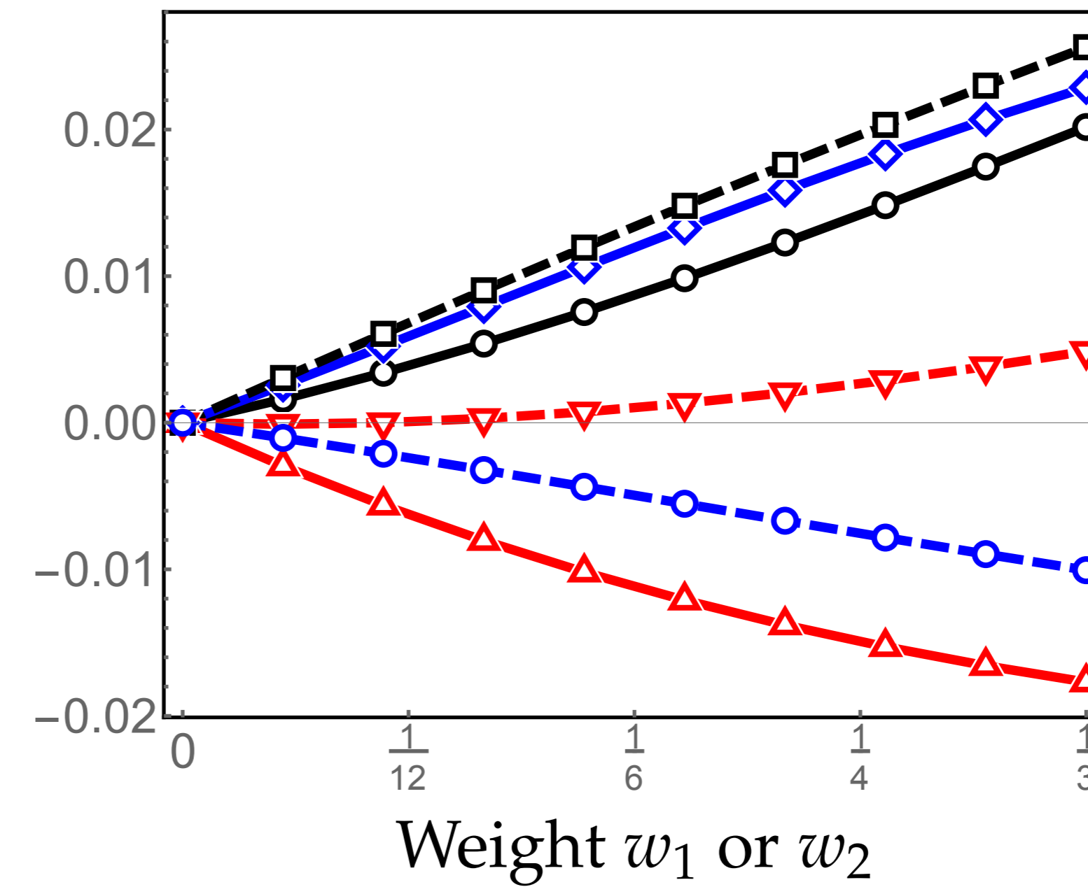
N = 5 and L = 8\pi
