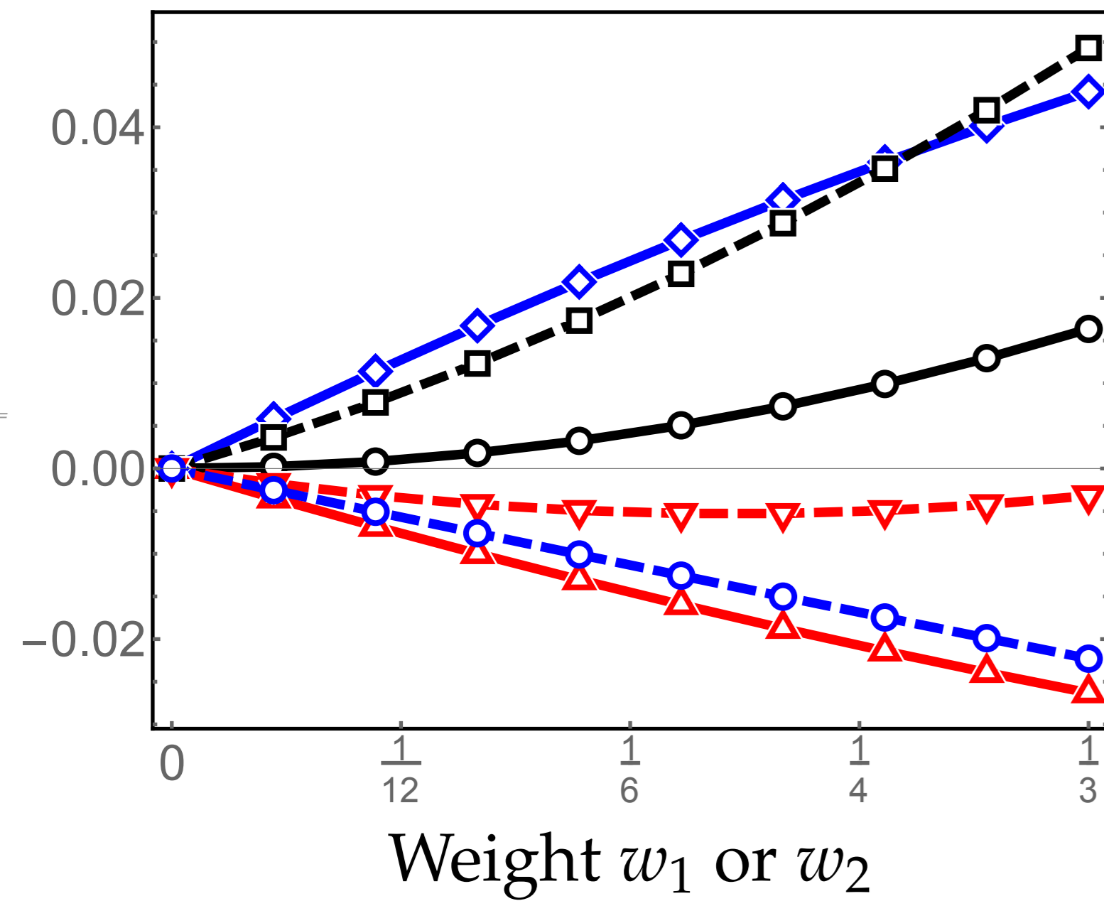
N = 5 and L = \pi/8
