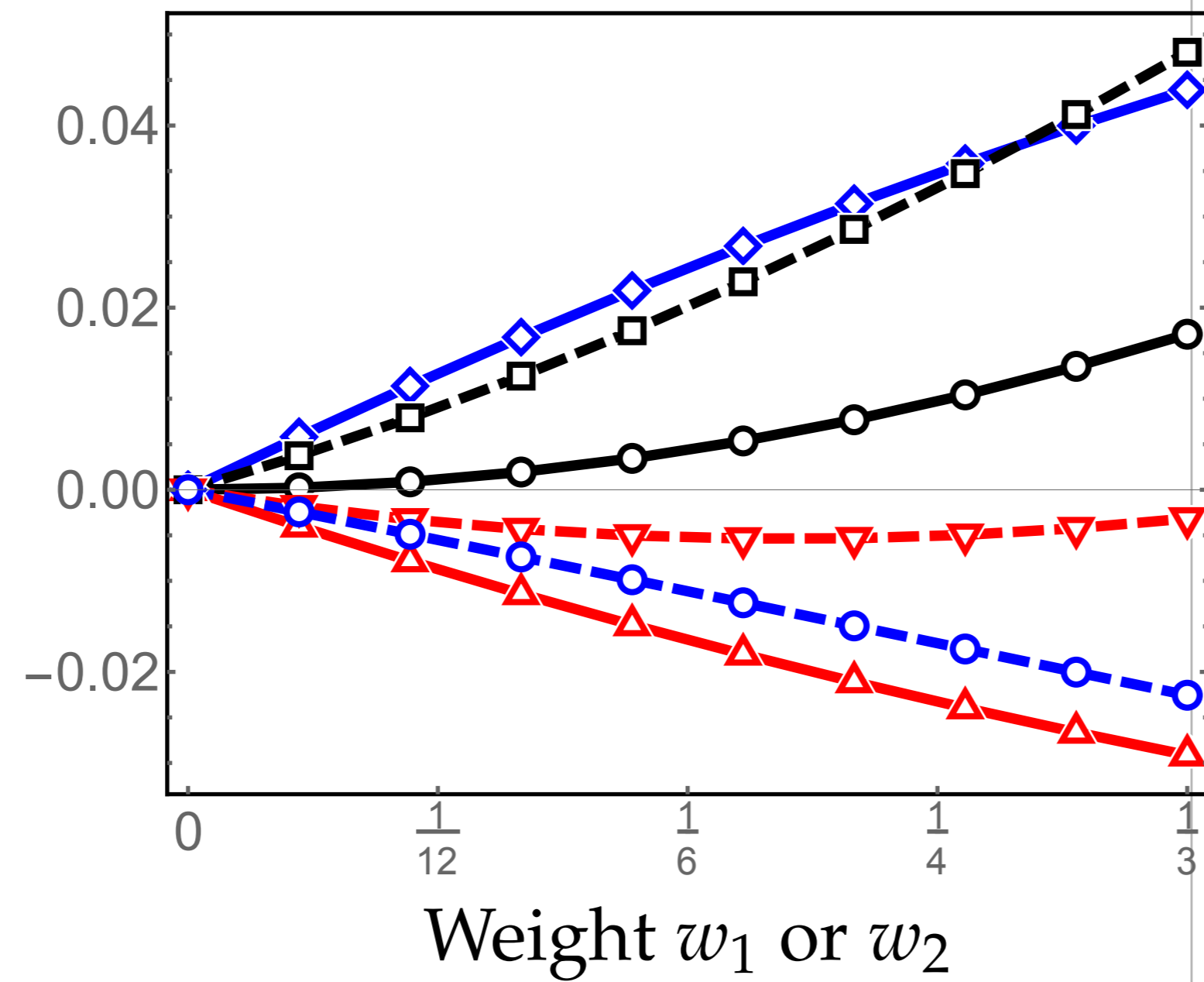
N = 5 and L = \pi
