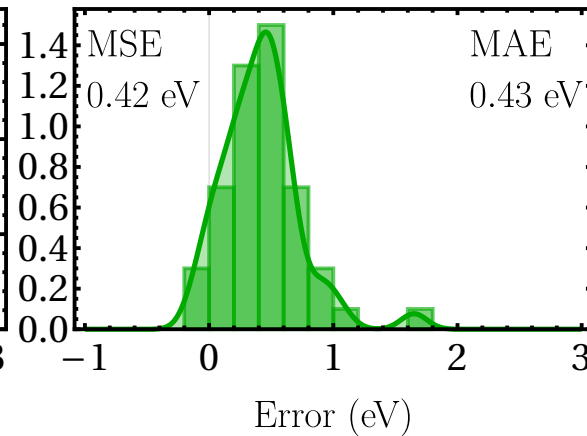
SRG-evGW@HF ( s = 1000 )
