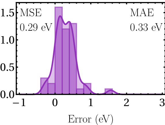
G_0W_0@HF ( \eta = 0.001 )
