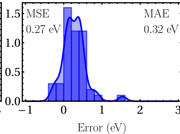
evGW@HF ( \eta = 0.1 )
