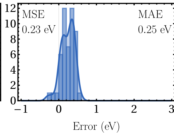
qsGW ( \eta = 0.1 )
