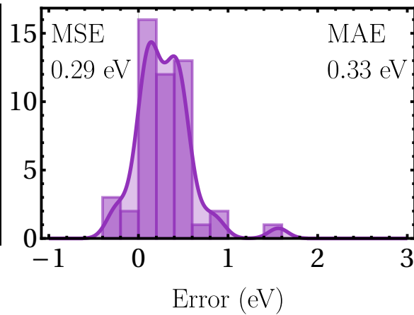
G_0W_0@HF ( \eta = 0.001 )
