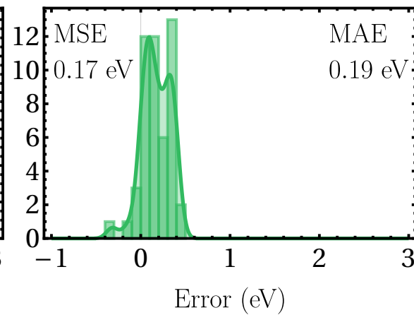
SRG-qsGW ( s = 1000 )
