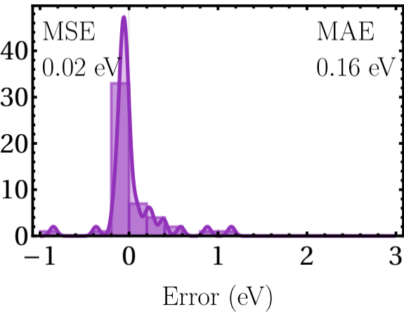
G_0W_0@HF ( \eta = 0.001 )
