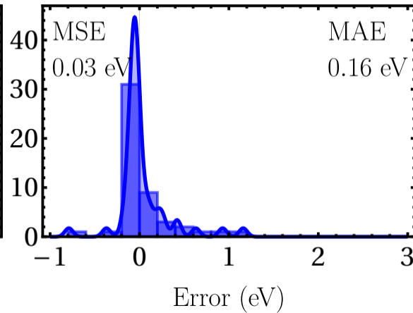
evGW@HF ( \eta = 0.1 )
