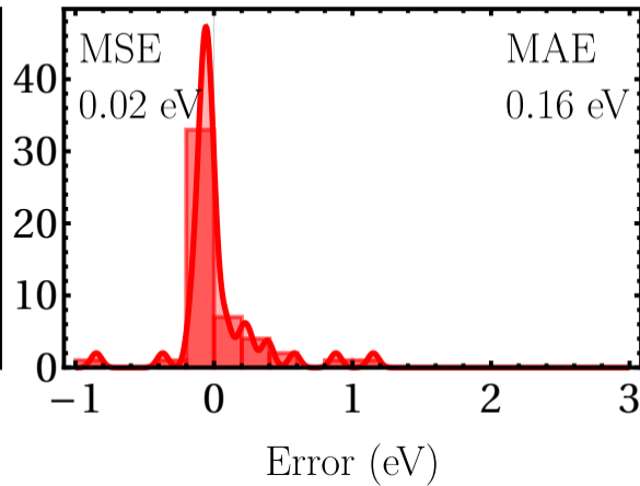
SRG- G_0W_0@HF ( s = 1000 )
