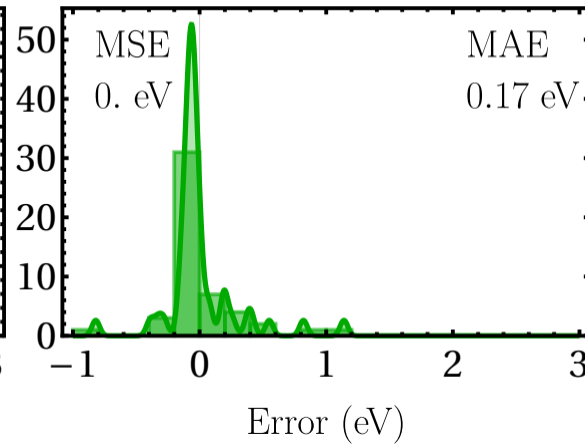
SRG-evGW@HF ( s = 50 )
