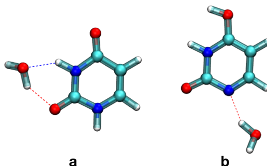
Figure 3.18: Structure of two (\text{H}_2\text{O})\text{U} isomers used for binding energy calculations.
