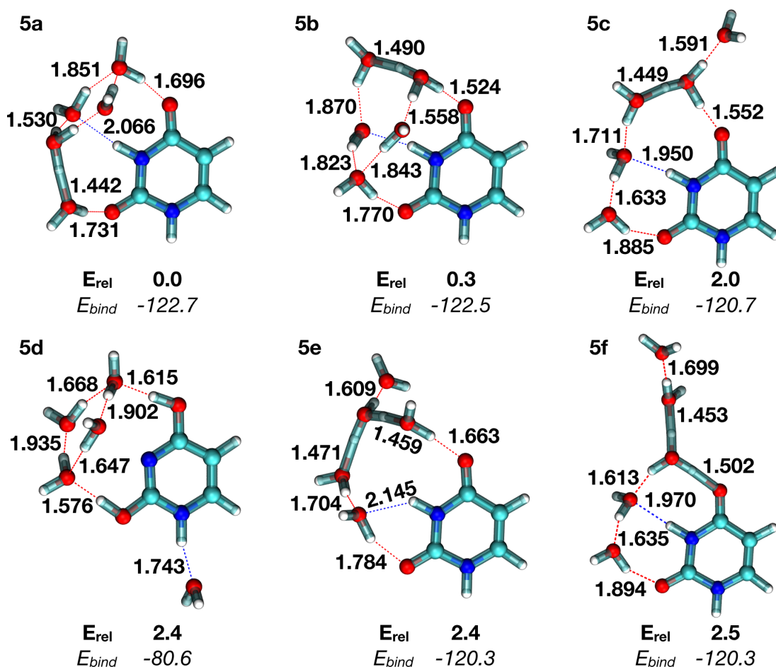
Figure 3.23: Lowest-energy structures of (\text{H}_2\text{O})_5\text{UH}^+ obtained at the MP2/Def2TZVP level of theory. Relative ( E_{rel} ) and binding energies ( E_{bind} ) are given in kcal.mol -1 . Important hydrogen-bond distances are indicated in bold and are given in Å.
