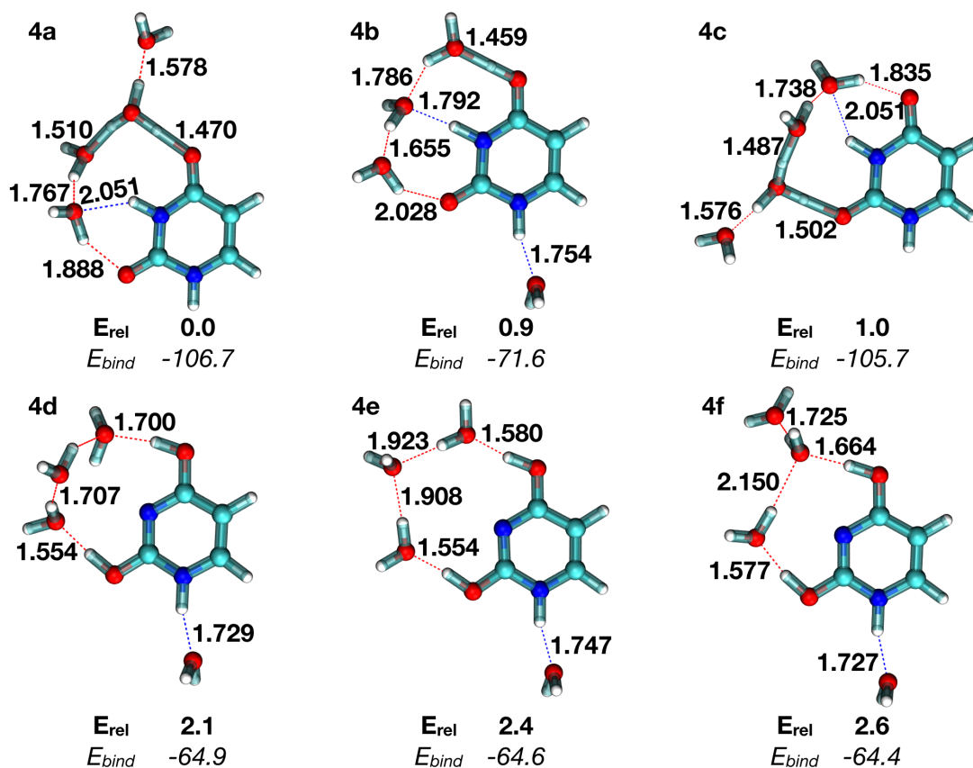
Figure 3.22: Lowest-energy structures of (\text{H}_2\text{O})_4\text{UH}^+ obtained at the MP2/Def2TZVP level of theory. Relative ( E_{rel} ) and binding energies ( E_{bind} ) are given in kcal.mol -1 . Important hydrogen-bond distances are indicated in bold and are given in Å.
