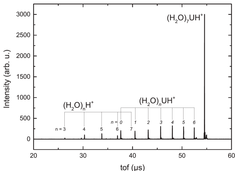
Figure 3.13: Time of flight of mass spectrum obtained by colliding (\text{H}_2\text{O})_7\text{UH}^+ with Ne at 7.2 eV center of mass collision energy (93.5 eV in the laboratory frame).
