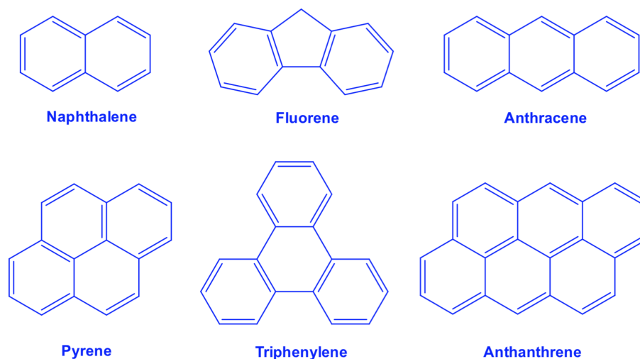
Figure 1.2: Examples of several PAH molecules.
