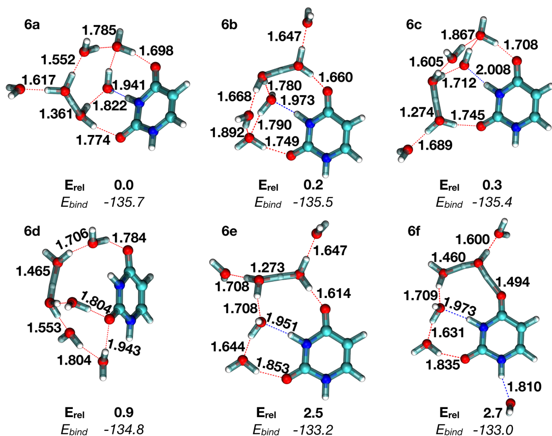
Figure 3.24: Lowest-energy structures of (\text{H}_2\text{O})_6\text{UH}^+ obtained at the MP2/Def2TZVP level of theory. Relative ( E_{rel} ) and binding energies ( E_{bind} ) are given in \text{kcal}\cdot\text{mol}^{-1} . Important hydrogen-bond distances are indicated in bold and are given in Å.
