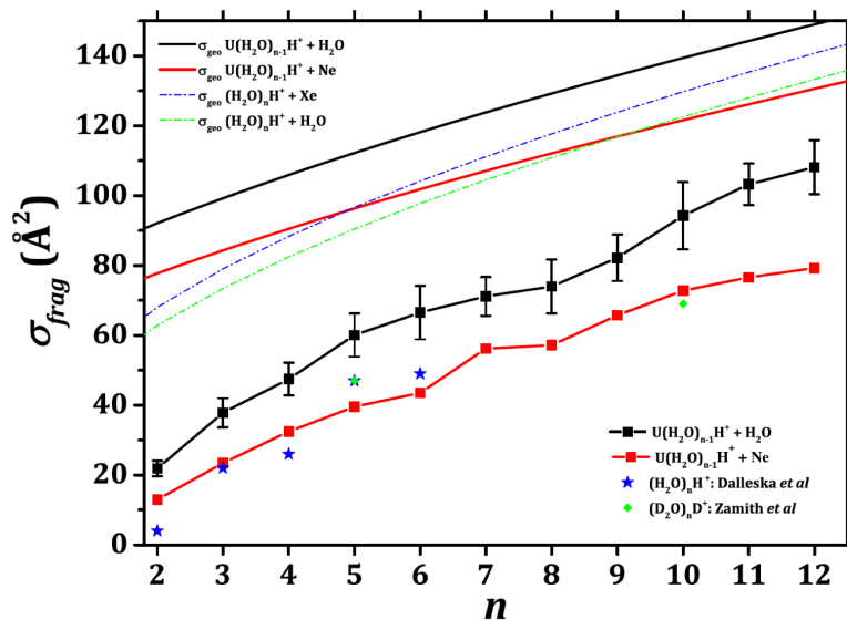
Figure 3.14: Fragmentation cross sections of clusters (H_2O)_{n-1}UH^+ at a collision energy of 7.2 eV plotted as a function of the total number n of molecules in the clusters. The experimental results and geometrical cross sections are shown for collision with H_2O and Ne. The results from N. Dalleska et al. [409] using Xe as target atoms on pure protonated water clusters (H_2O)_{2-6}H^+ and from S. Zamith et al. [410] using water as target molecules on deuterated water clusters (D_2O)_{5,10}H^+ are also shown. The geometrical collision cross sections of water clusters in collision with Xe atoms and water molecules are also plotted. Error bars represent one standard deviation.
