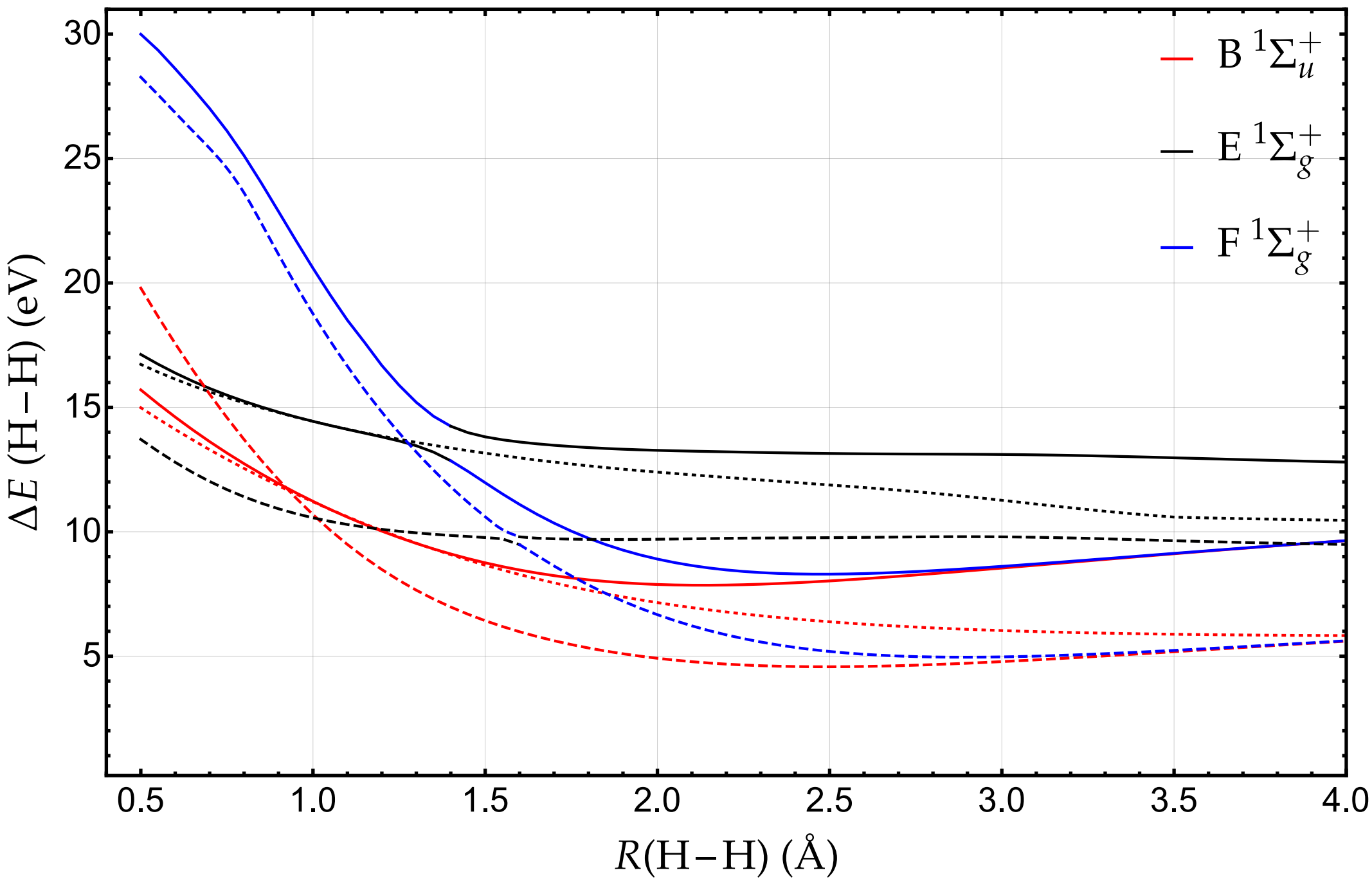
(SF-)TD-LC- \omega PBE08 vs EOM-CCSD
