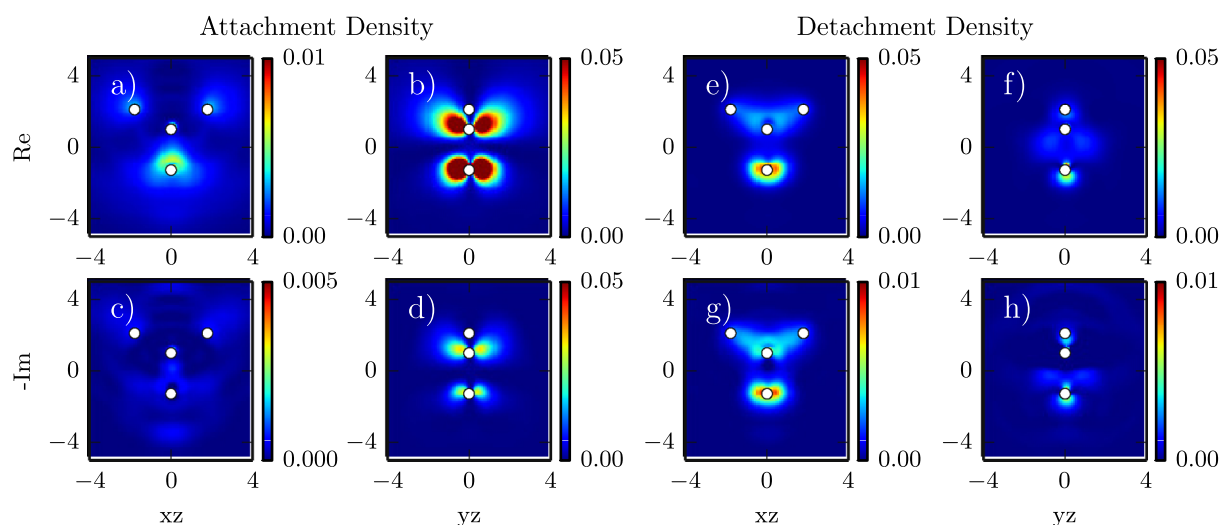
FIG. 2. Real and imaginary parts of the \alpha attachment and detachment densities for the ^2B_1 resonance in formaldehyde are plotted in the xz and yz -planes. The top row shows the real part and the bottom row shows the negative of the imaginary part. The first four panels (a)-(d) show the attachment density while the second four (e)-(h) show the detachment density. Note the difference in scales. White dots are used to indicate the positions of the nuclear centers and the oxygen end of the molecule points in the negative z -direction. The axes are in atomic units ( a_0 ). The real and imaginary parts of the attachment density, which correspond to the extra electron in the resonance state, are predominantly \pi^* in character. The detachment density, which corresponds to rearrangement, has largely \sigma character.
