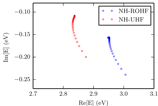
FIG. 1. Representative \theta -trajectories for \text{N}_2^- in the caug-cc-pVDZ(cm+) basis set. The complex basis function parameter, \theta , is varied from 10^\circ to 25^\circ in increments of 0.5^\circ . The approximate location of the stationary point is (2.8, -0.1) for NH-UHF, while for NH-ROHF, it is (2.9, -0.15).
