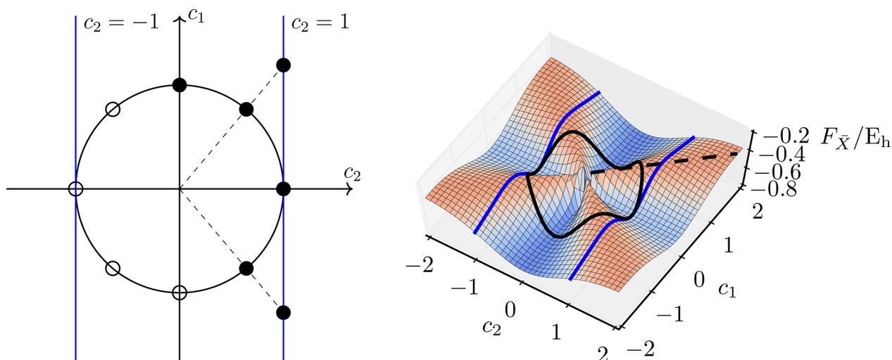
Figure 1. Constrained projective h-RHF energy F_{\bar{X}} for the n = 2 system H_2 (STO-3G) at a bond length of 2.5 Å. The coordinate c_0 defines the normalization constant, representing the distance of a point from the origin, and \frac{\partial F_{\bar{X}}}{\partial c_0} = 0 for all c_0 \neq 0 . Exploiting this invariance, every stationary point constrained to the circle c_1^2 + c_2^2 = 1 (black curve) with c_2 \neq 0 can also be located as a stationary point constrained to the line c_2 = 1 (blue line), where rescaling recovers the normalized h-RHF state (dashed line). Because of the overall sign symmetry, only half the stationary points need to be considered (filled circles vs open circles).
