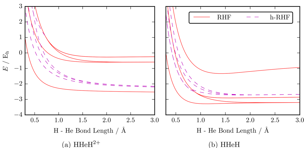
Figure 6. Thirteen h-RHF states for (a) \text{HHeH}^{2+} and (b) \text{HHeH} in STO-3G for a range of symmetric H–He bond lengths. Six solutions have complex coefficients across all bond lengths, arising in degenerate complex-conjugate pairs. At around 0.7 Å in \text{HHeH}^{2+} and around 0.9 Å in \text{HHeH} , two pairs of complex solutions coalesce to form a 4-fold degenerate set of complex h-RHF states.
