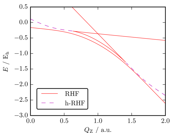
Figure 5. Four h-RHF solutions of HZ (STO-3G) are plotted against the nuclear charge Q_Z for a bond length of 2.50 Å, showing the smooth interconversion between the complex h-RHF states of \text{HHe}^+ (at Q_Z = 2.00 au) and \text{H}_2 (at Q_Z = 1.00 au). Two h-RHF states of \text{HHe}^+ that exist with complex coefficients for all bond lengths are seen to smoothly interconvert with real h-RHF states of \text{H}_2 as Q_Z is varied.
