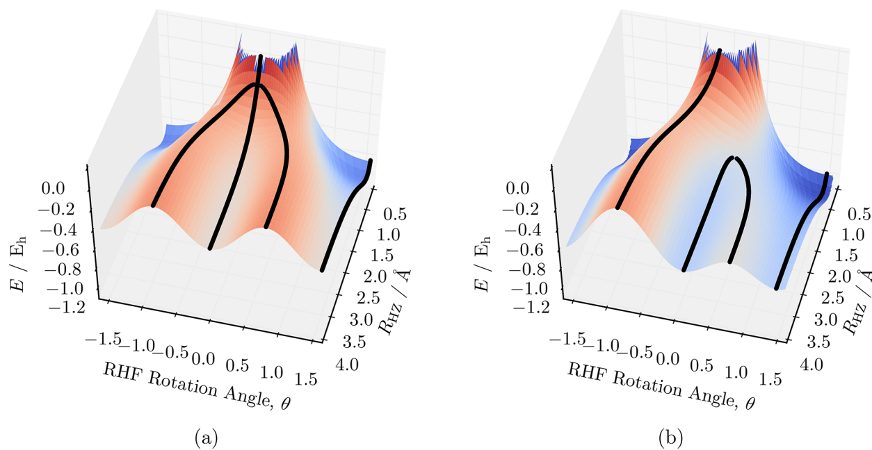
Figure 4. Conventional Hartree–Fock energy plotted as a function of the RHF rotation angle, \theta (eq 23) for Q_Z = 1.00 au and Q_Z = 1.15 au. (a) When Q_Z = 1.00 au the molecule possesses D_{\infty h} symmetry and the ionic solutions simultaneously converge with the \sigma_u^2 state, disappearing at a triply degenerate A_3 cusp catastrophe in a pitchfork bifurcation. (b) For Q_Z = 1.15 au the molecular symmetry becomes C_{\infty v} , decomposing the pitchfork bifurcation into a primary branch and two secondary modes that coalesce and disappear at a doubly degenerate A_2 fold catastrophe.
