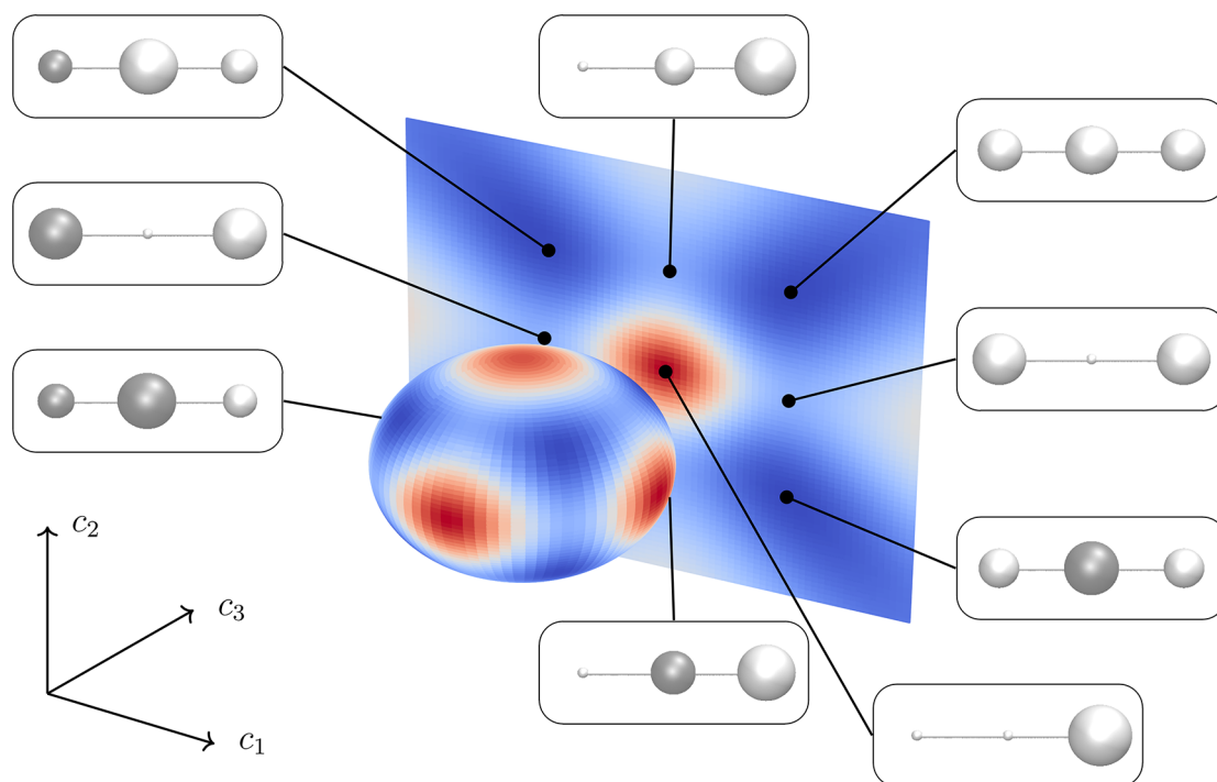
Figure 2. Constrained projective h-RHF energy F_{\bar{X}} plotted on the sphere c_1^2 + c_2^2 + c_3^2 = 1 and the plane c_3 = 1 for linear H_3^+ (STO-3G) at a bond length of 2.5 Å. Nine stationary points can be located on the plane c_3 = 1 , as shown alongside their corresponding orbital plots. The remaining four h-RHF states exist at the infinities of this plane, and can be located by finding the stationary points constrained to the plane c_3 = 0 . The bond length has been chosen such that all solutions and their energies are real, although the results extend to geometries where complex h-RHF states are present.
