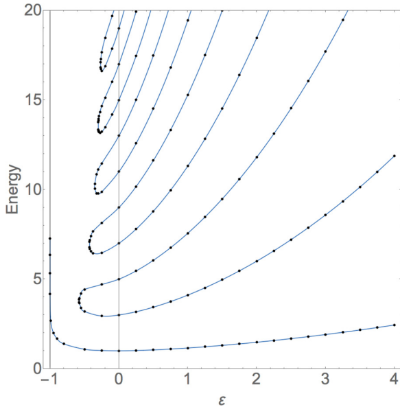
FIG. 1. Real eigenvalues of the Hamiltonian H = p^2 + x^2(ix)^\epsilon plotted as functions of the parameter \epsilon . When \epsilon \geq 0 (the region of unbroken \mathcal{PT} symmetry), the spectrum is real, positive, and discrete. However, as \epsilon goes below 0 ( \epsilon < 0 is known as the region of broken \mathcal{PT} symmetry ) the real eigenvalues begin to merge pairwise and form complex-conjugate pairs. When -1 < \epsilon < 0 , there are only a finite number of real positive eigenvalues and an infinite number of complex-conjugate pairs of eigenvalues. When \epsilon \leq -0.57793 , only one real eigenvalue survives and as \epsilon approaches -1^+ , this real eigenvalue becomes infinite. The behavior of the complex eigenvalues in the region of broken \mathcal{PT} symmetry is not shown in this graph and has not been explored until now.
