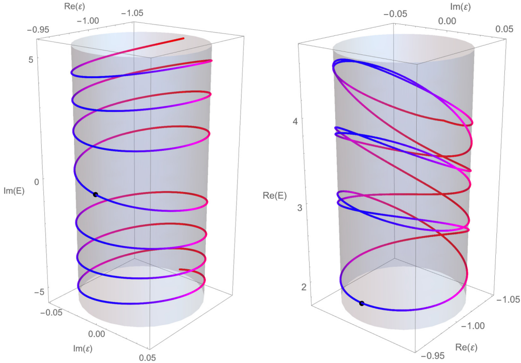
FIG. 5. Behavior of the eigenvalues of the Hamiltonian H = p^2 + x^2(ix)^\epsilon as the parameter \epsilon winds around the exceptional point at \epsilon = -1 in a circle of radius 0.05 in the complex- \epsilon plane. This singular point is an infinite-order exceptional point, and all of the complex eigenvalues analytically continue into one another as one encircles the exceptional point. The lines are shaded blue when \text{Re } \epsilon > -1 and red when \text{Im } \epsilon < -1 . The behavior of the imaginary parts of the eigenvalues (left panel) are easier to visualize because they exhibit a simple logarithmic spiral. The dot shows that the imaginary part of an eigenvalue (the eigenvalue shown in black in Figs. 3 and 4) vanishes (the eigenvalue is real) when \text{Re } \epsilon > -1 . However, as we wind in one direction the imaginary parts of the eigenvalues increase in a helical fashion and as we wind in the opposite direction the imaginary parts of the eigenvalues decrease in a helical fashion. As we pass the real- \epsilon axis we pass through the values plotted on the red dashed lines shown in Figs. 3 and 4. A shaded cylinder has been drawn to assist the eye in the following this helix. The behavior of the real parts of the eigenvalues (right panel) is more complicated because the curves form a double helix . The two helices intersect 4 times each time the singular point at \epsilon = -1 is encircled, and they intersect at 90^\circ intervals. If we begin at the dot, then we see that the real parts of the eigenvalues increase as we rotate about \epsilon = -1 in either direction. Each time \epsilon crosses the real axis in the complex- \epsilon plane the curves pass through the values shown at the left and right edges of Fig. 4.
