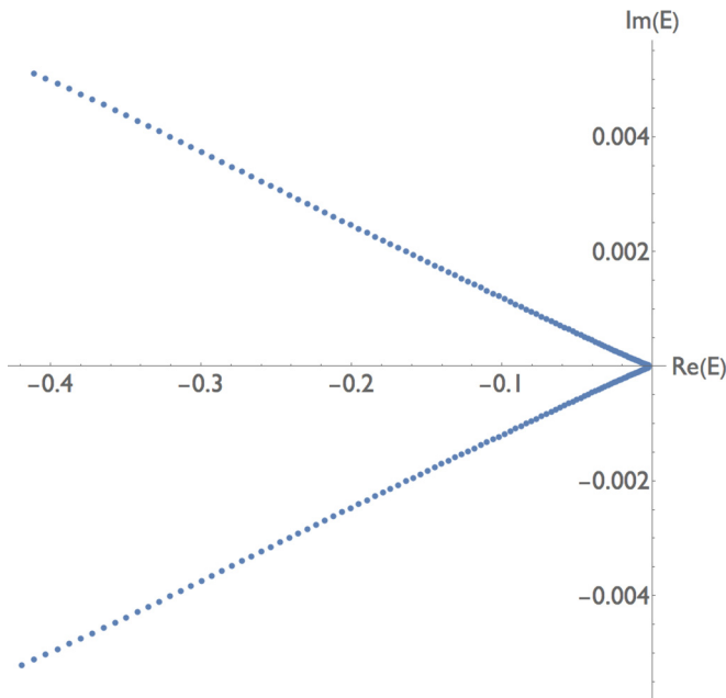
FIG. 16. Detail of the region around the origin in the complex eigenvalue plane of Fig. 15 for \epsilon = -3 . For this figure we have chosen \eta = 0.999 and have taken the very small cell size 0.00001.
