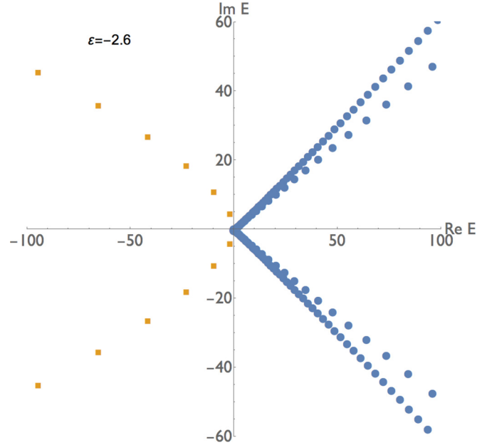
FIG. 11. Discrete and continuous parts of the spectrum of the \mathcal{PT} -symmetric Hamiltonian H = p^2 + x^2(ix)^\epsilon for the case \epsilon = -2.6 . The discrete eigenvalues (orange squares) occur in pairs in the left-half complex plane. The continuous eigenvalues (blue dots) lie on two complex-conjugate pairs of curves in the right-half complex plane. As we decrease the cell size in the Arnoldi algorithm, the dots become dense on these curves. The continuous curves of eigenvalues originate slightly to the left of the origin.
