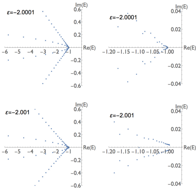
FIG. 10. Eigenvalues of the Hamiltonian H = p^2 + x^2(ix)^\epsilon for \epsilon = -2.0001 and -2.001 . (The right panels are magnifications of the left panels.) The spectrum lies in the left-half complex plane and is partly continuous and partly discrete. The eigenvalues in the continuous part of the spectrum lie on a pair of complex-conjugate curves that radiate away from -1 and as we calculate more eigenvalues, the points on these curves become denser. The discrete part of the spectrum consists of eigenvalues lying on two complex-conjugate curves that are much closer to the negative-real axis. There is an elaborate structure near \epsilon = -1 . As \epsilon goes below -2 , the eigenvalues move away from -1 ; specifically, for \epsilon = -2.0001 the distance from -1 to the nearest eigenvalue is about 0.0005 and for \epsilon = -2.001 the distance to the nearest eigenvalue is about 0.008 .
