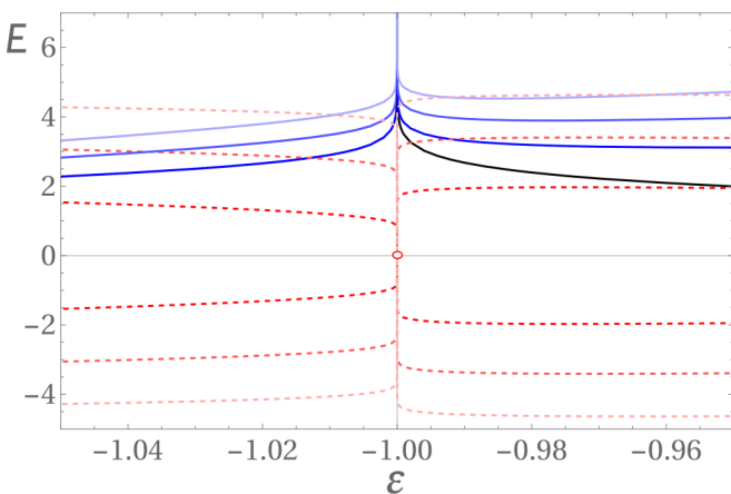
FIG. 4. Detailed view of Fig. 3 showing the behavior of the eigenvalues of the Hamiltonian H = p^2 + x^2(ix)^\epsilon plotted as functions of the parameter \epsilon for -1.05 \leq \epsilon \leq -0.95 . There is one real eigenvalue for \epsilon > -1 (solid black line). The real parts of the complex eigenvalues (blue solid lines) and the real eigenvalue diverge at \epsilon = -1 . The complex eigenvalues occur in complex-conjugate pairs and the imaginary parts of the eigenvalues rapidly go to 0 at \epsilon = -1 . These behaviors are expressed quantitatively in (14).
