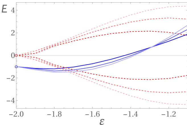
FIG. 6. First three complex-conjugate pairs of eigenvalues of the Hamiltonian H = p^2 + x^2(ix)^\epsilon plotted as functions of \epsilon for -2 \leq \epsilon \leq -1.1 . This figure is a continuation of Fig. 3. Note that the real parts of the eigenvalues coalesce to -1 and the imaginary parts coalesce to 0 as \epsilon approaches -2 . The results of a WKB calculation of these eigenvalues near \epsilon = -2 is given in (29). Note that the real parts of the eigenvalues cross near \epsilon = -1.3 , but they do not all cross at the same point as can be seen in Fig. 7.
