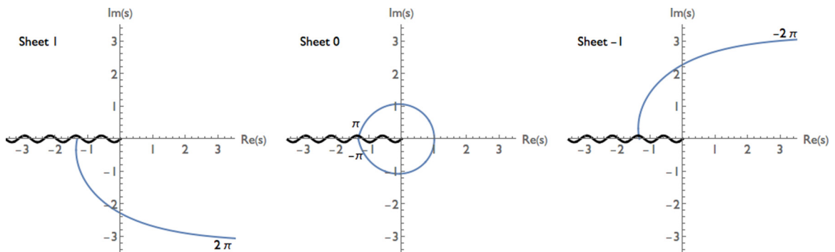
FIG. 8. Contour in the complex- s plane for the complex Coulomb potential \epsilon = -3 . The contour comes in from \infty parallel to the positive-real axis at an angle of -2\pi in the center of the left Stokes wedge (right panel). Next, it loops around the origin in the positive direction (center panel). Finally, it goes back out to \infty parallel to the positive-real axis at an angle of 2\pi in the center of the right Stokes wedge (left panel). The total rotation about the origin is 4\pi .
