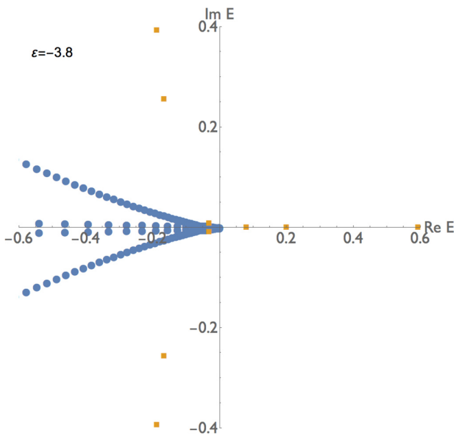
FIG. 17. Eigenspectrum for \epsilon = -3.8 . The continuous part of the spectrum (blue dots) lies on two complex-conjugate pairs of curves in the left-half plane and resembles that of the Coulomb case (see Fig. 15). The discrete part of the spectrum (orange squares) consists of complex-conjugate eigenvalues in the left-half plane and real eigenvalues on the positive-real axis.
