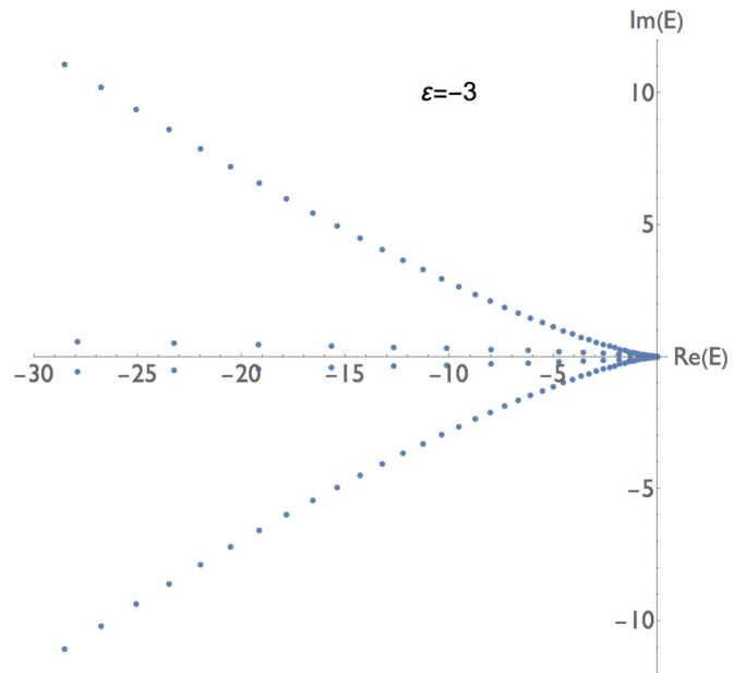
FIG. 15. Eigenvalues for the Coulomb case \varepsilon = -3 . There are no discrete eigenvalues and the continuum eigenvalues lie on four curves in the left-half complex plane.
