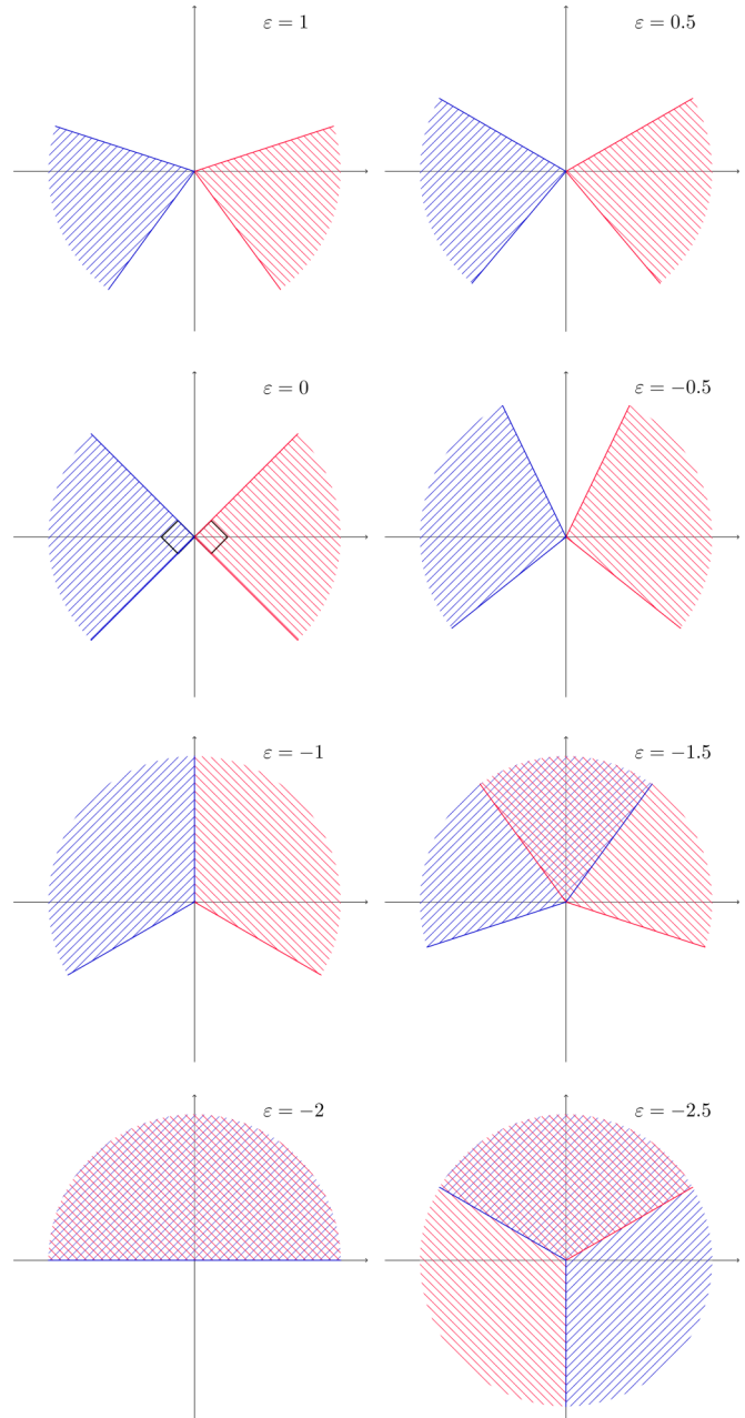
FIG. 2. Stokes wedges associated with the eigenvalue problem for the Hamiltonian H = p^2 + x^2(ix)^\varepsilon for eight values of \varepsilon . The locations of center lines, the upper edges, and the lower edges of the Stokes wedges are given in (3)–(5). The left wedge is blue and the right wedge is red. As \varepsilon decreases, the wedges get wider and rotate upwards. At \varepsilon = -1 the two wedges touch and fuse into one wedge. However, when \varepsilon goes below -1 , the sheets are again distinct; the left wedge rotates clockwise into sheet -1 and the right wedge rotates anticlockwise into sheet 1 .
