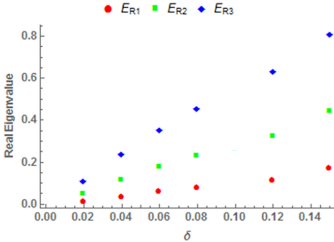
FIG. 19. First three real eigenvalues of the Hamiltonian H = p^2 + x^2(ix)^\epsilon plotted as functions of the parameter \delta , where \epsilon = -4 + \delta . The eigenvalues clearly approach 0 as \delta \rightarrow 0 and we see strong evidence that the eigenvalues vanish linearly with \delta .
