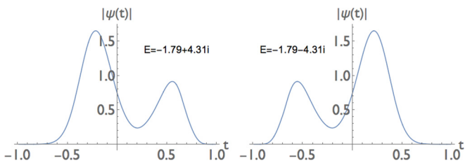
FIG. 13. Absolute values of the eigenfunctions \psi(t) for the discrete eigenvalues -1.79 \pm 4.31i for \varepsilon = -2.6 . The eigenfunctions satisfy homogeneous boundary conditions at \pm(1 - \eta) for \eta = 0.01 and look like bound-state eigenfunctions in the sense that the eigenfunctions decay to 0 exponentially fast at both boundary points. The left and right panels are interchanged under t \rightarrow -t , which corresponds to a \mathcal{PT} reflection.
