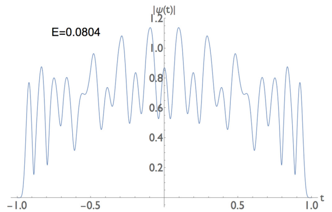
FIG. 18. Plot of the absolute value of the eigenfunction associated with the discrete real eigenvalue E = 0.0804 for \epsilon = -3.8 .
