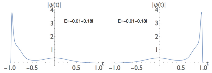
FIG. 14. Absolute values of the eigenfunctions for the continuum eigenvalues -0.01 \pm 0.18i for \varepsilon = -2.6 . These eigenvalues belong to the continuous spectrum. The indication that they are part of the continuous spectrum is that at one of the boundary points the eigenfunctions suddenly drop to 0 rather than decaying exponentially to 0. As in Fig. 13, the left and right panels are interchanged under t \rightarrow -t , which corresponds to a \mathcal{PT} reflection.
