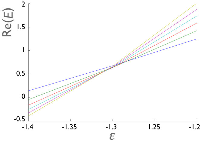
FIG. 7. Detail of Fig. 6 showing the behavior of the real parts of the first six eigenvalues of the Hamiltonian H = p^2 + x^2(ix)^\epsilon for -1.4 \leq \epsilon \leq -1.2 . The real parts of the eigenvalues cross almost at the same value of \epsilon but the imaginary parts of the eigenvalues remain well separated.
