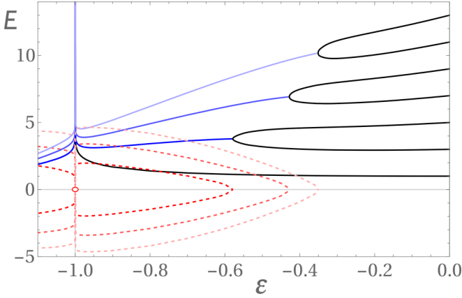
FIG. 3. Eigenvalues of the Hamiltonian H = p^2 + x^2(ix)^\epsilon plotted as functions of the parameter \epsilon for -1.1 < \epsilon < 0 . This graph is a continuation of the graph in Fig. 1. As \epsilon decreases below 0 and enters the region of broken \mathcal{PT} symmetry, real eigenvalues (solid black lines) become degenerate and then form complex-conjugate pairs. The real parts of these pairs of eigenvalues (solid blue lines) initially decrease as \epsilon decreases but blow up suddenly as \epsilon approaches -1 . The real parts then decrease as \epsilon decreases below -1 . The imaginary parts of the eigenvalue pairs (dashed red lines) remain finite and appear to suffer discontinuous jumps at \epsilon = -1 . However, a closer look shows that these dashed lines rapidly decay to 0 near \epsilon = -1 and then rapidly come back up to different values as \epsilon passes through -1 . A blow-up of the region near \epsilon = -1 is given in Fig. 4.
