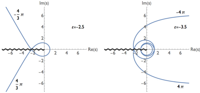
FIG. 9. Eigenvalue contours in the complex- s plane for the cases \epsilon = -2.5 and \epsilon = -3.5 .
