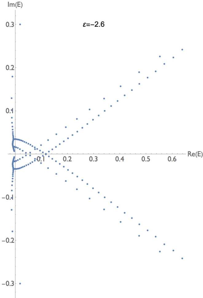
FIG. 12. Detail of Fig. 11 showing the elaborate structure of the spectrum near the origin in the complex-eigenvalue plane for \varepsilon = -2.6 .
